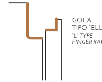
ANTA CON PROFILO AD "ELLE" DOOR WITH "L-SHAPED" PROFILE
