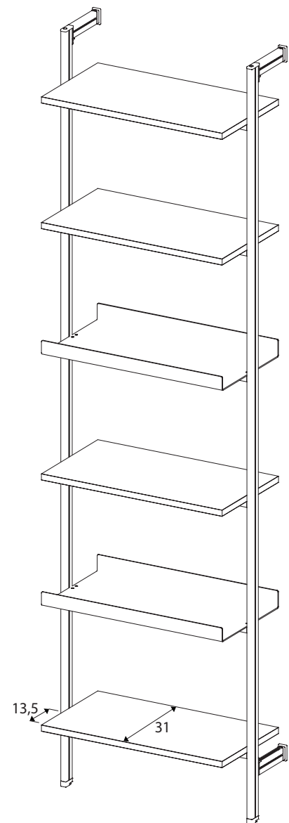
sporgenza mensola shelf protrusion
