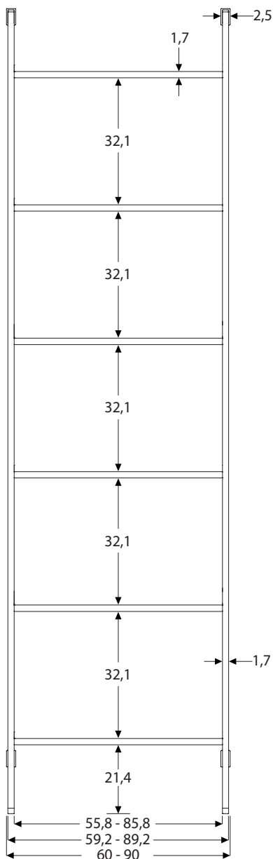
VISTA FRONTALE FRONT VIEW
