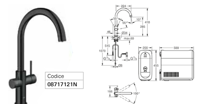
Blue Home | bocca C
