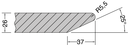
PROFILO SVASATO STONDATEO ROUNDED FLARED PROFILE
