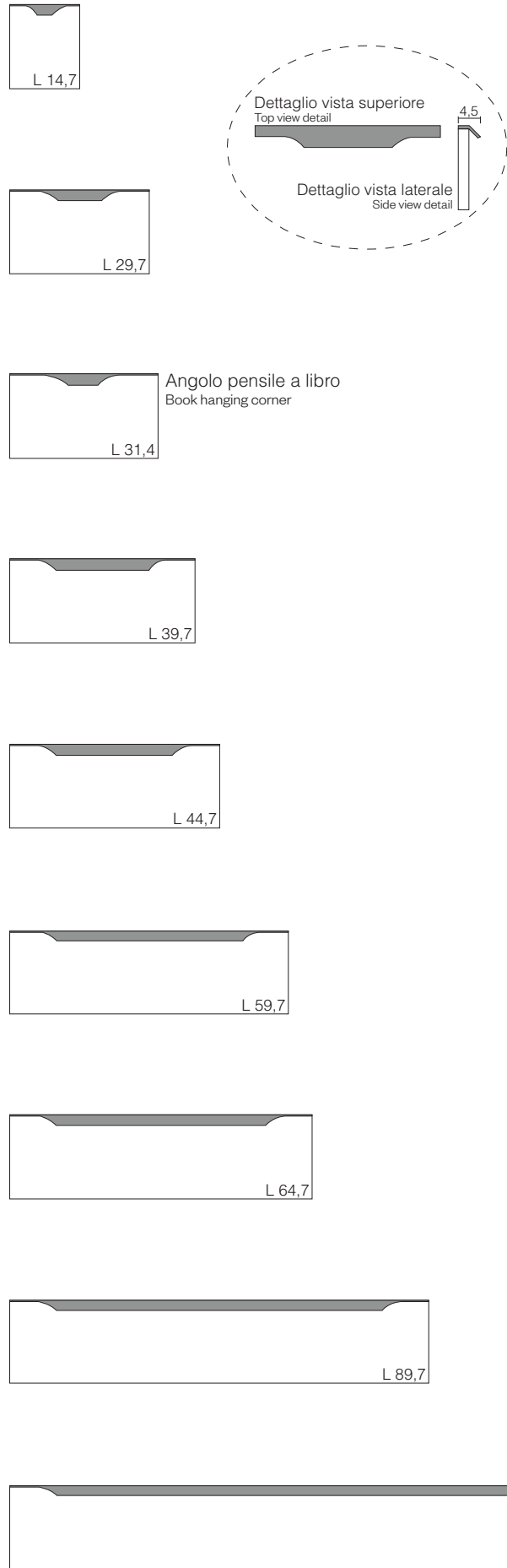
MANIGLIA APPLICATA IN TESTA TOP-MOUNTED HANDLE
