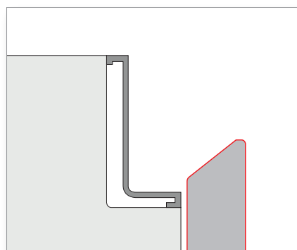
ANTA INCLINATA SENZA PROFILO INCLINED DOOR WITHOUT PROFILE
