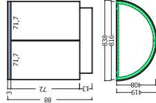
ISOLA/PENISOLA CIRCOLARE ROUND ISLAND/PENINSULA UNIT
