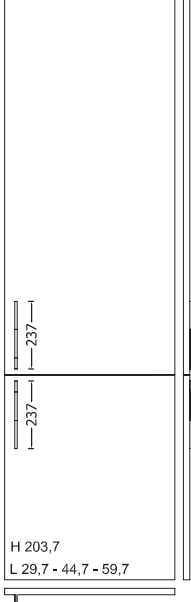
FRIGO - DISPENSA 1 ANTA COLUMN FRIDGE - CABINET
