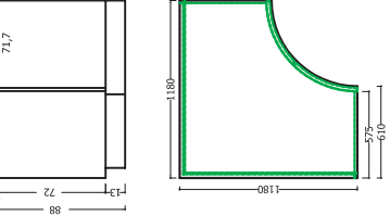
ANGOLO BASE 118 X 118 CORNER BASE UNIT
