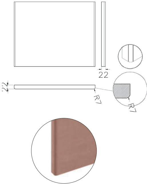
particolare anta detail of door
