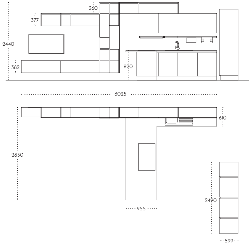
BASI - PENSILI - LIVING / BASE UNITS - WALL UNITS - LIVING
